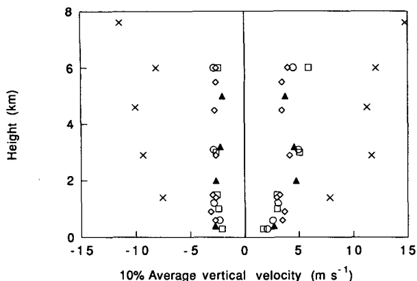
FIG. 3. Comparison of strongest 10% level average vertical velocity in updraft and downdraft cores for EMEX (triangles), GATE (circles), hurricane rainbands (diamonds), TAMEX (squares), and the Thunderstorm Project (crosses). Adapted from Zipser and LeMone (1980).
